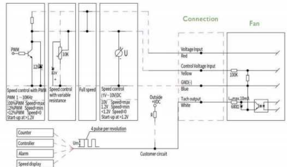
Customer Circuit
